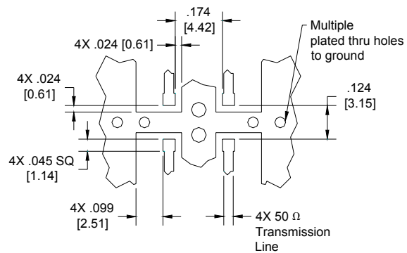
Dimensions are in Inches [Millimeters] JP503 Rev A Mounting Footprint
